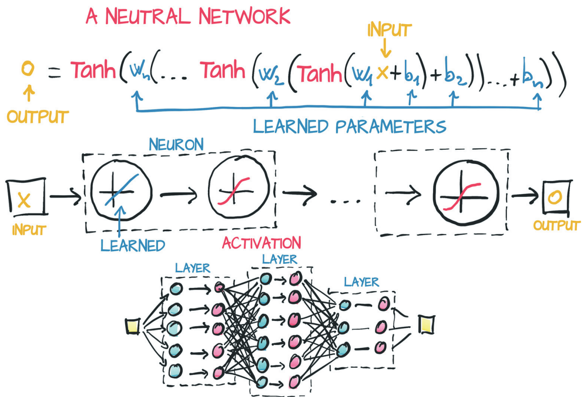
Figure 5.3 A neural network with three layers
